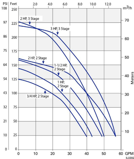
CJ101 BRASS IMPELLERS
